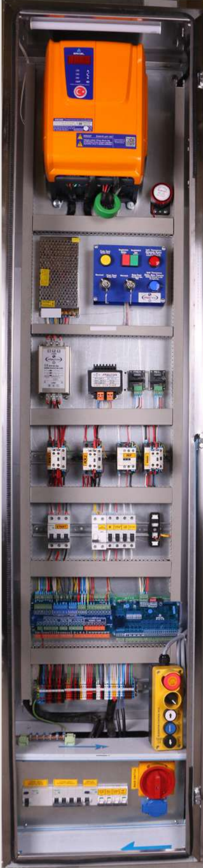
mrl dislisiz kontrol panosu (mrl gearless control board)
